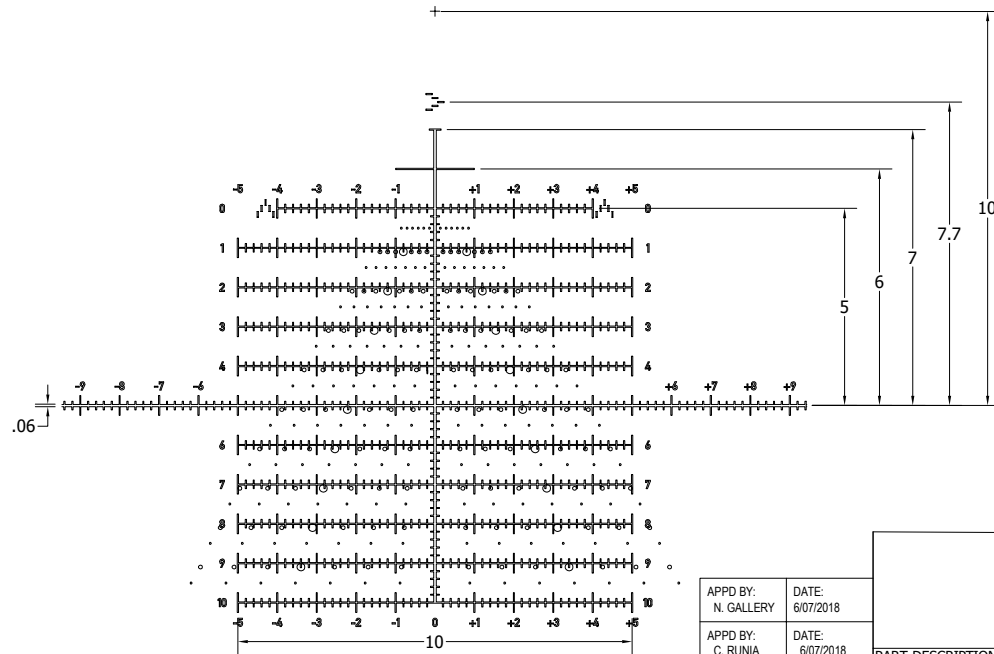
DETAIL D
