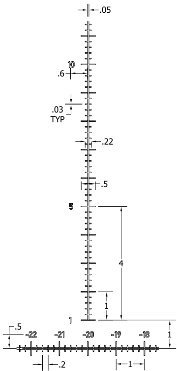
DETAIL C
